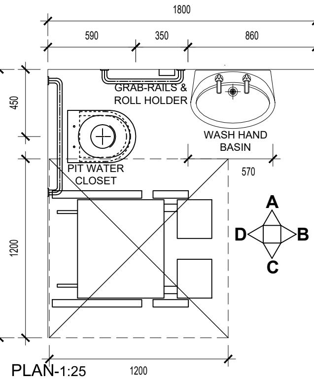
PLAN-1:25
