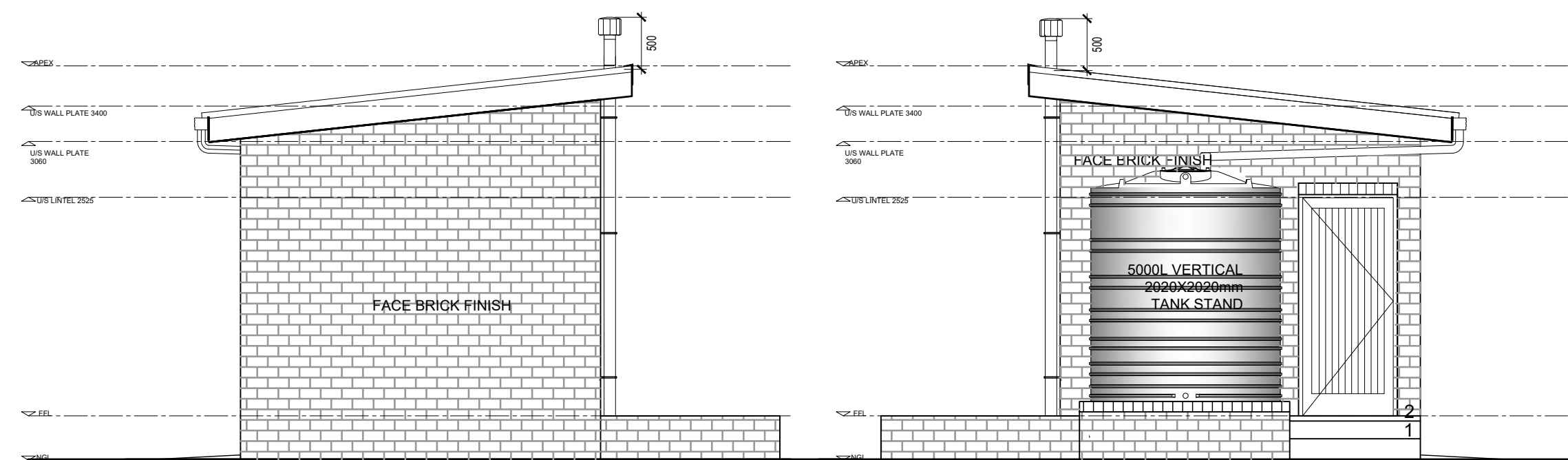
RIGHT ELEVATION SCALE 1:50
