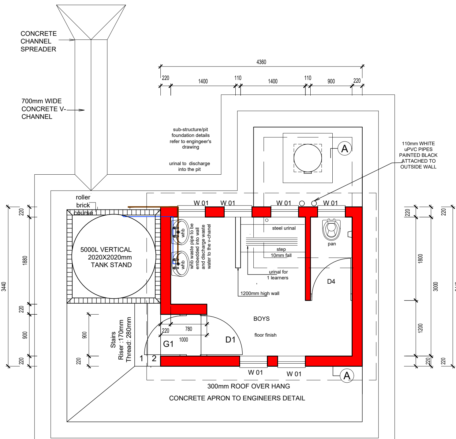
FLOOR PLAN SCALE 1:50
