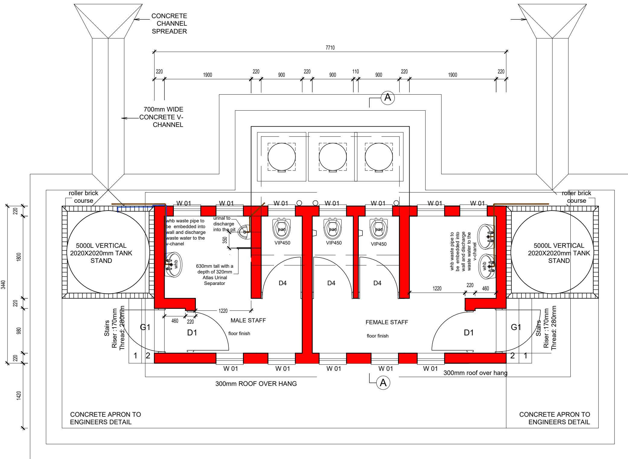
FLOOR PLAN SCALE 1:50
