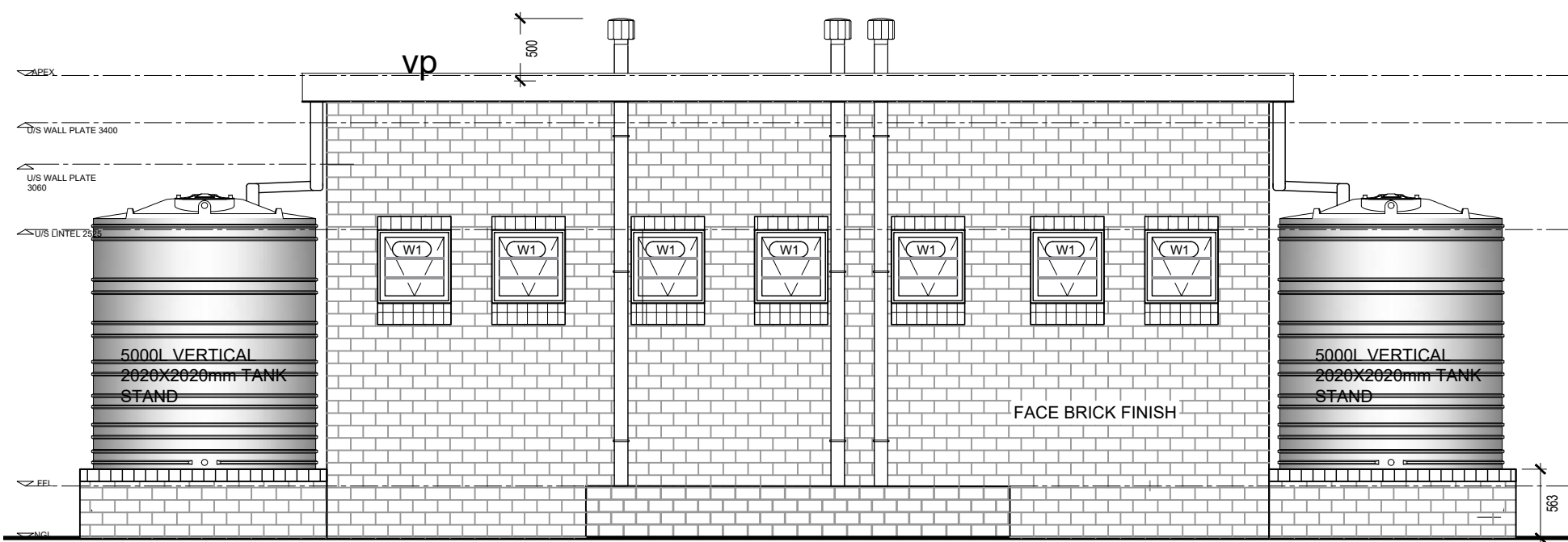
REAR ELEVATION SCALE 1:50
