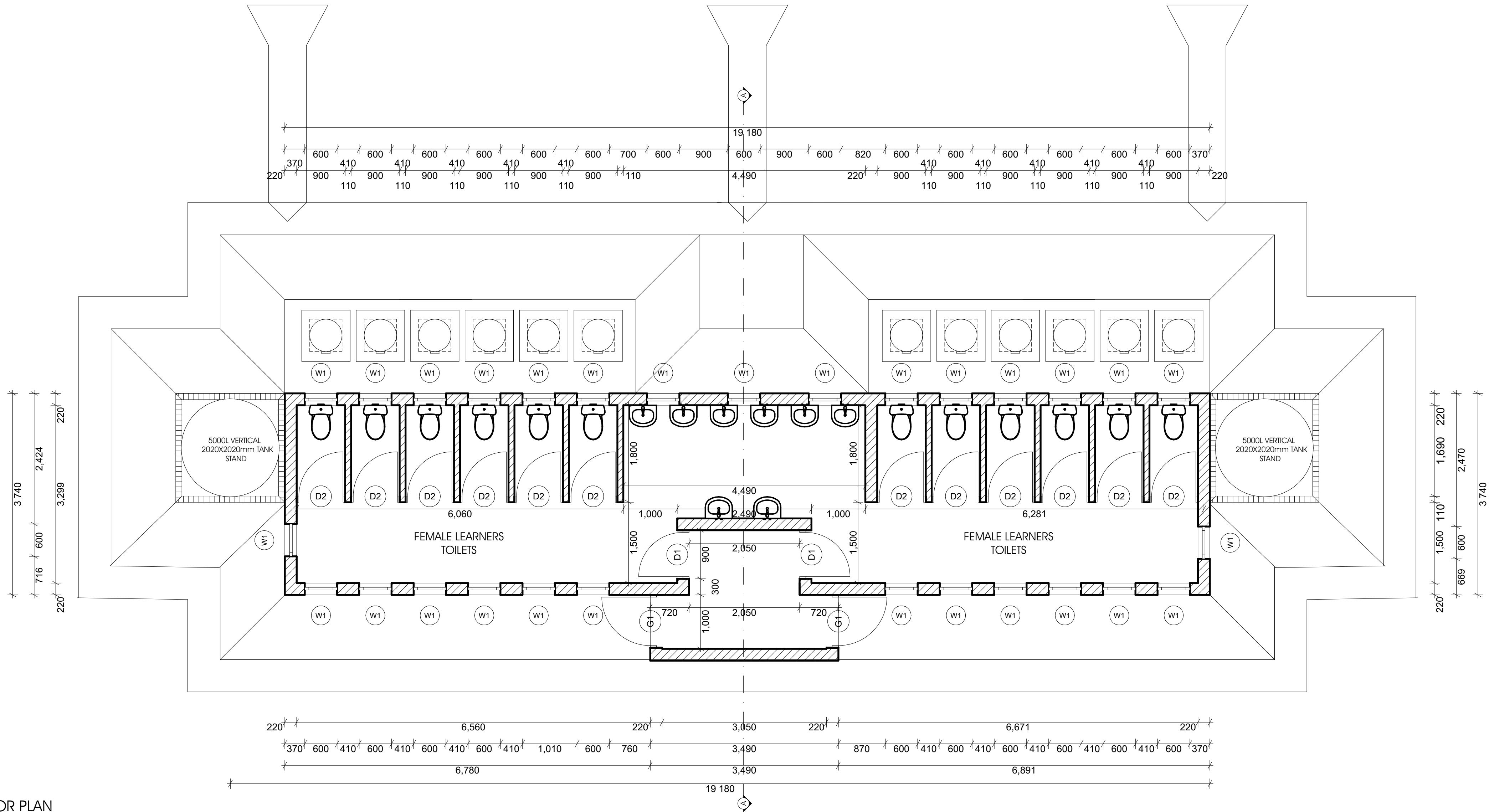
FLOOR PLAN SCALE 1:100
