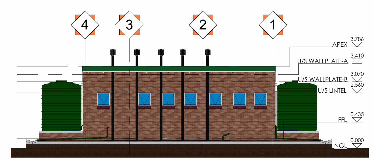
3 Siyabonga SSS - Staff Toilet North Elevation 1 : 100
