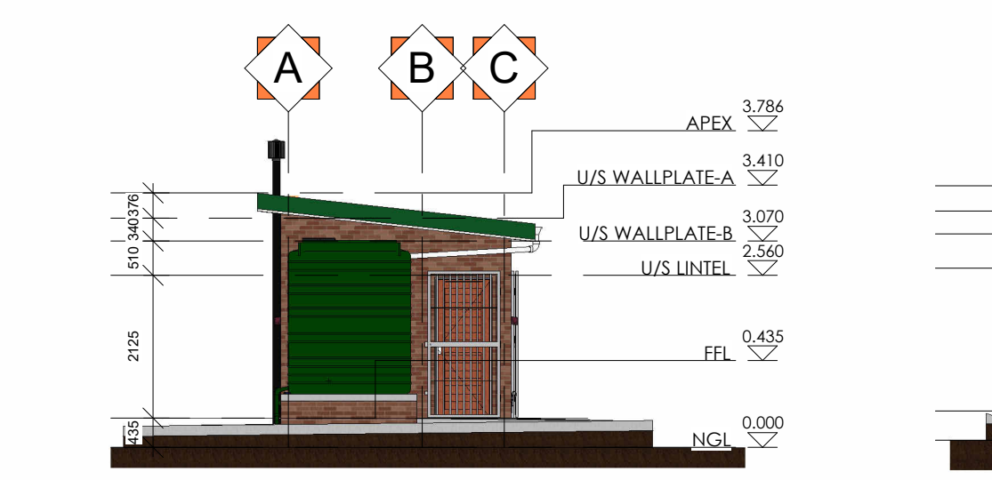
5 S - Staff Toilet West Elev. 1 : 100
