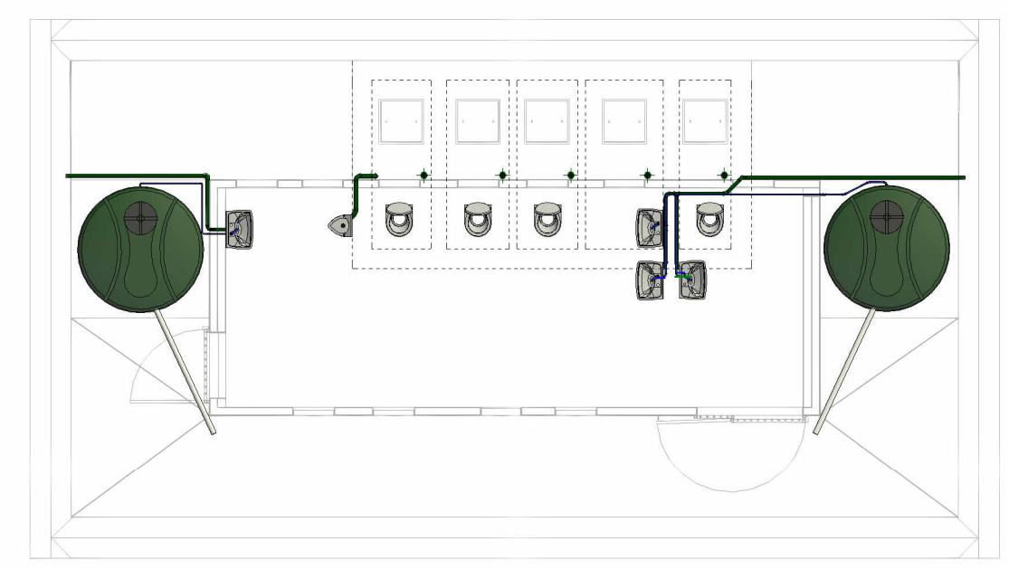
2 Staff Toilet - Plumbing Layout 1 : 100
