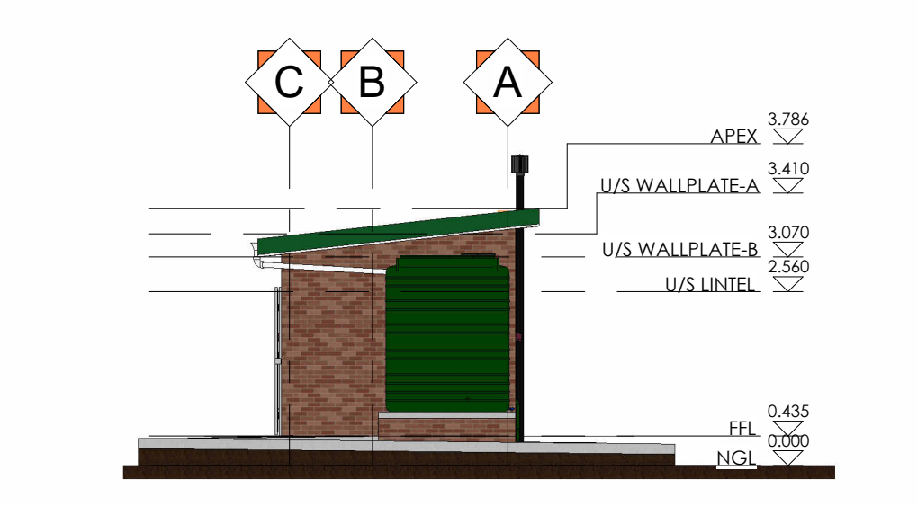
6 S - Staff Toilet East Elev. 1 : 100
