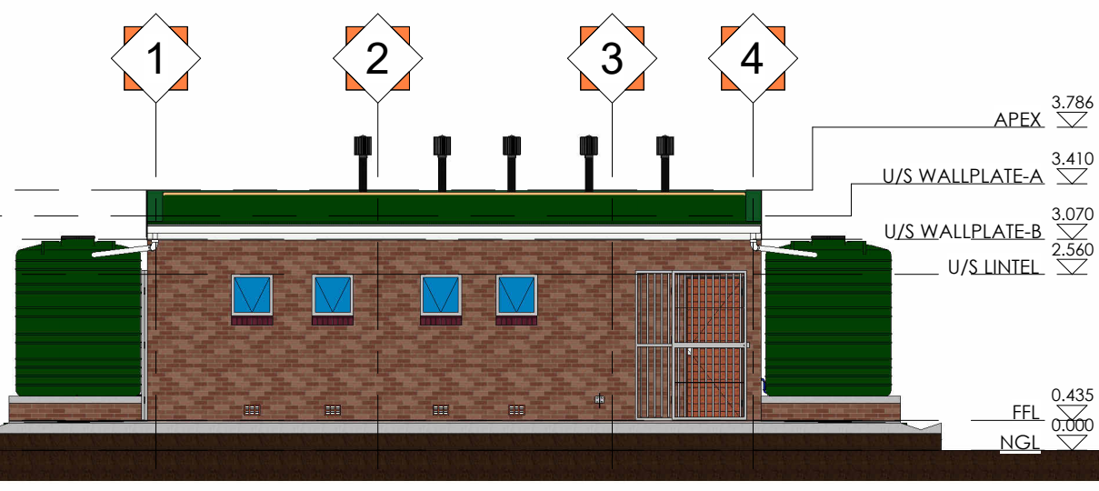
4 Siyabonga SSS - Staff Toilet South Elevation 1 : 100
