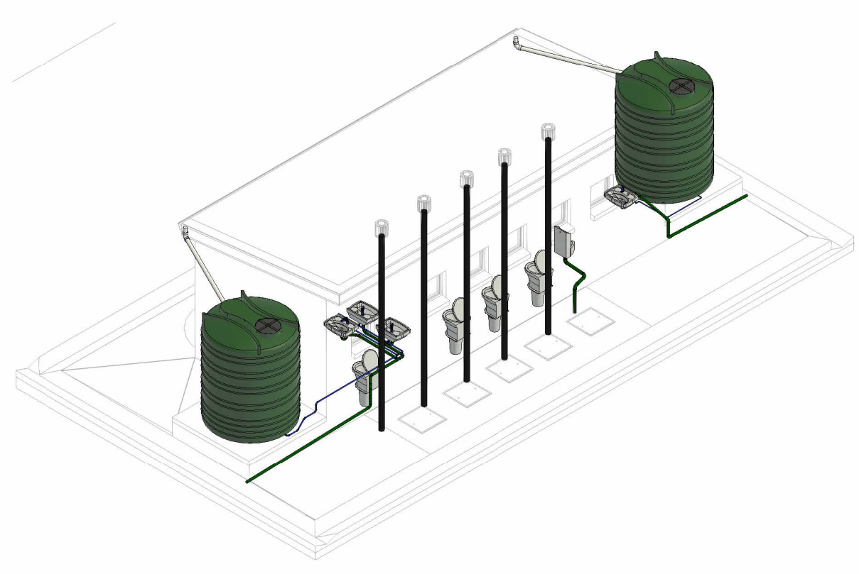
8 Plumbing - 3D View
