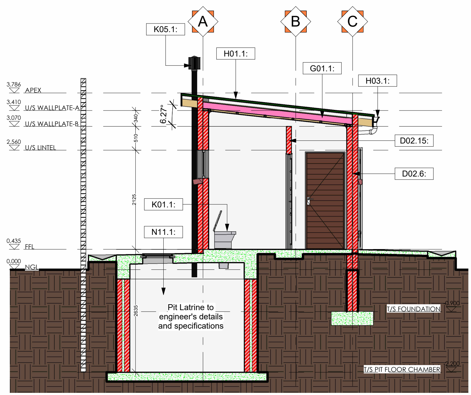
7 Siyabonga SSS - Staff Toilet - Cross Section 1 : 50
