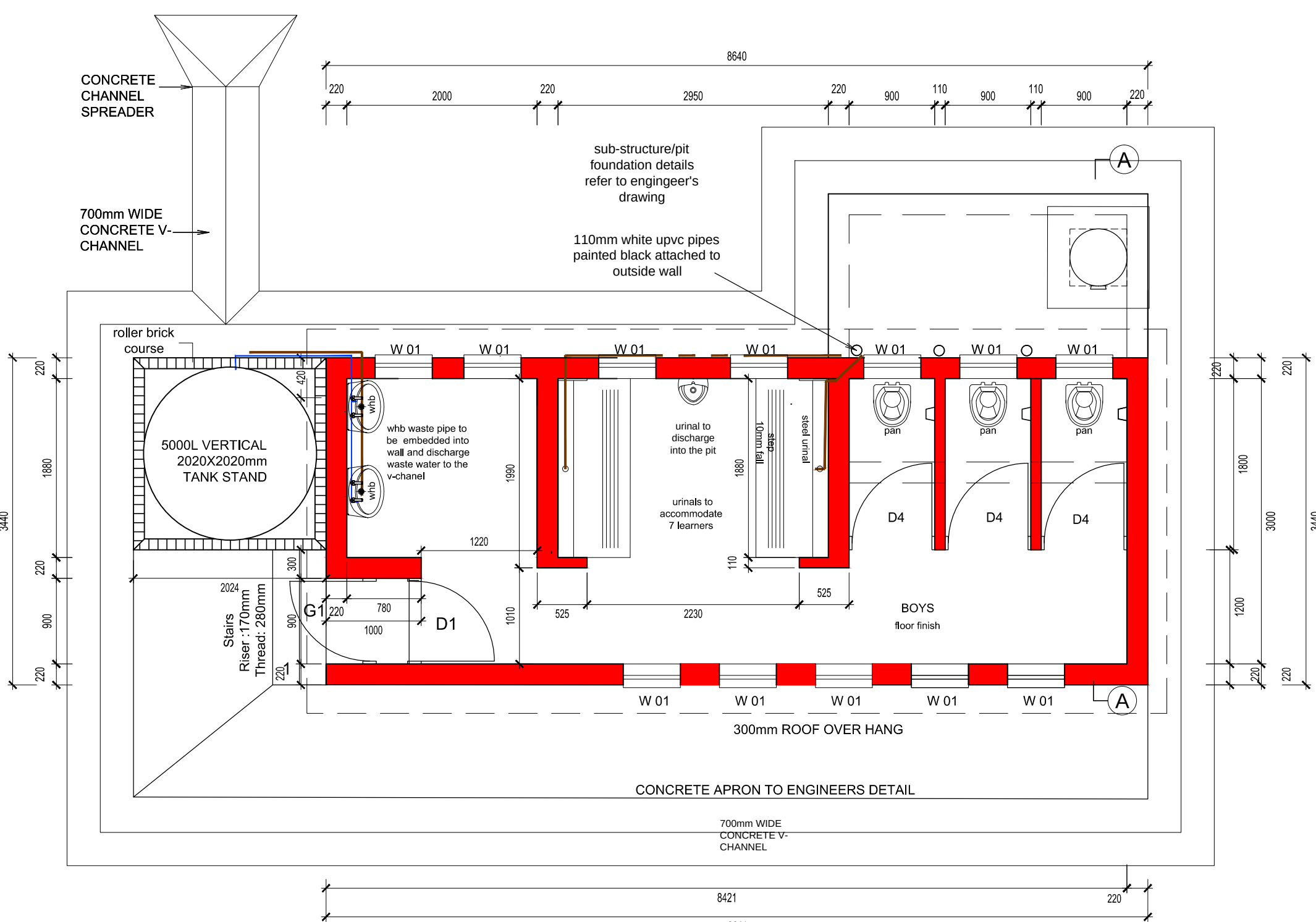
FLOOR PLAN SCALE 1:50
