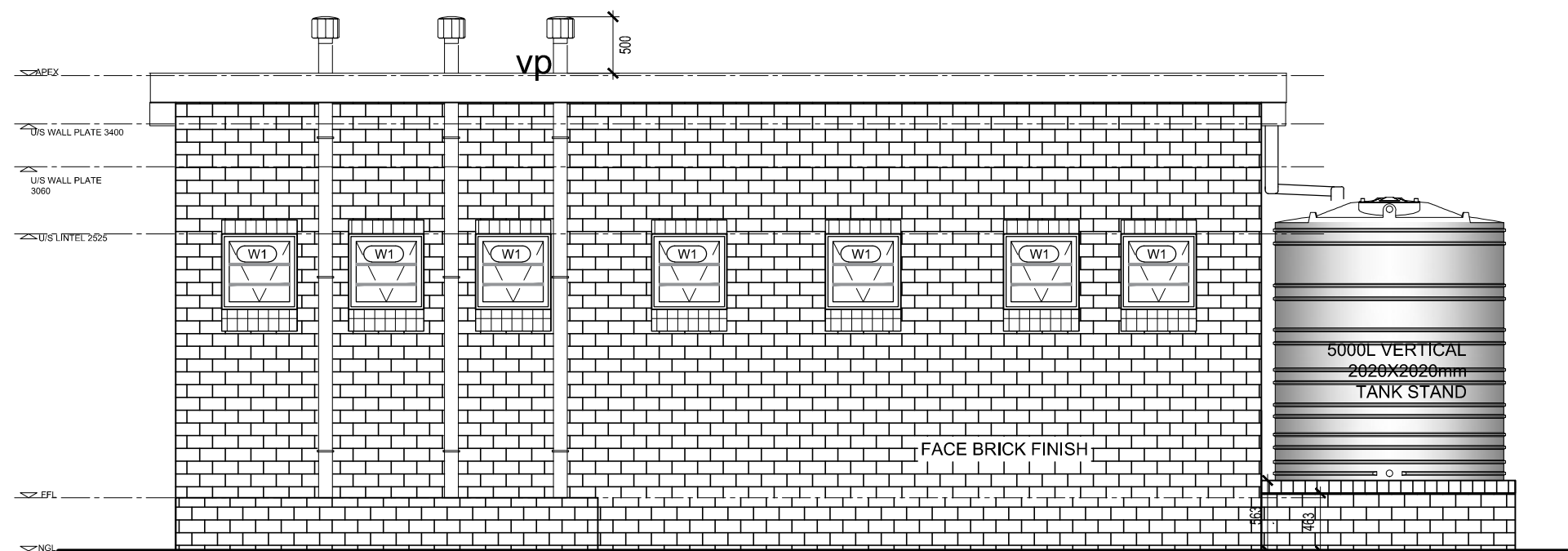
REAR ELEVATION SCALE 1:50
