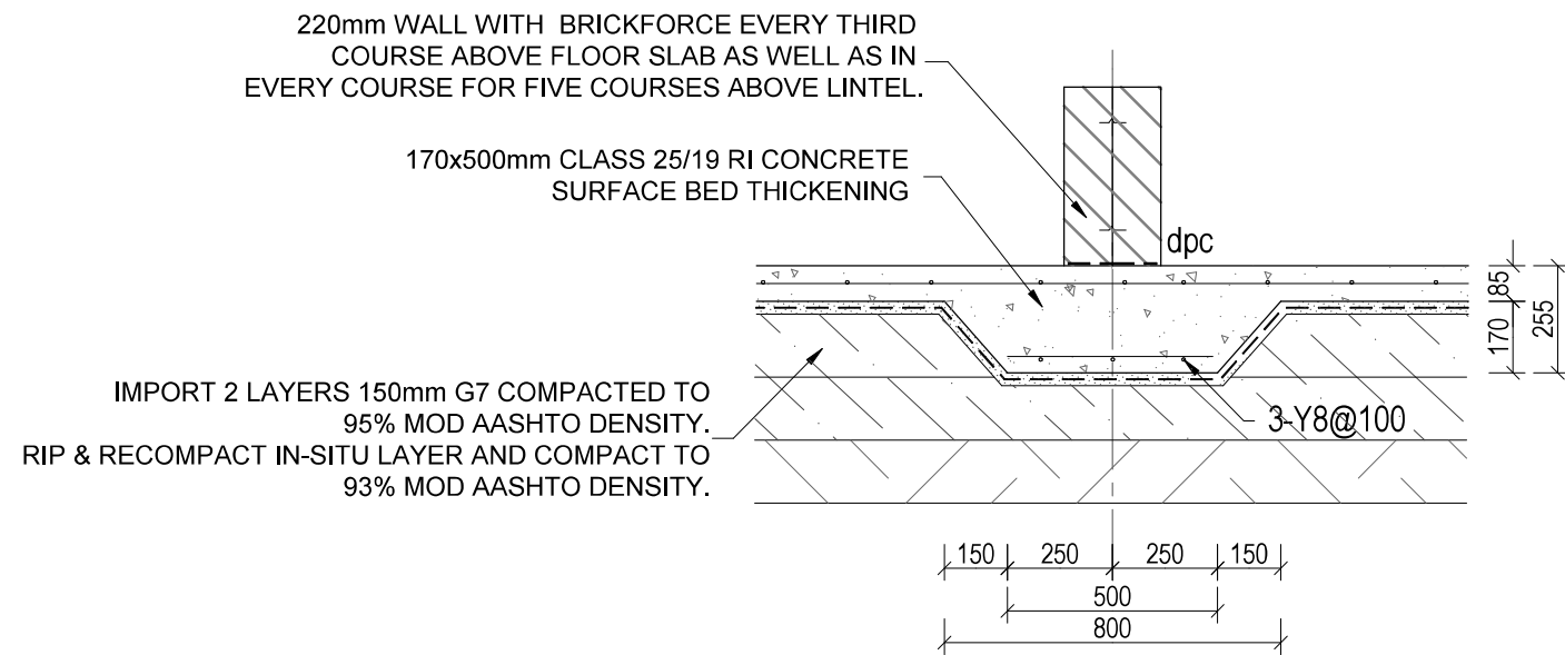
SURFACE BED THICKENING 220mm INTERNAL WALL with 170x500mm THICKENING SCALE 1:20 (A1)
