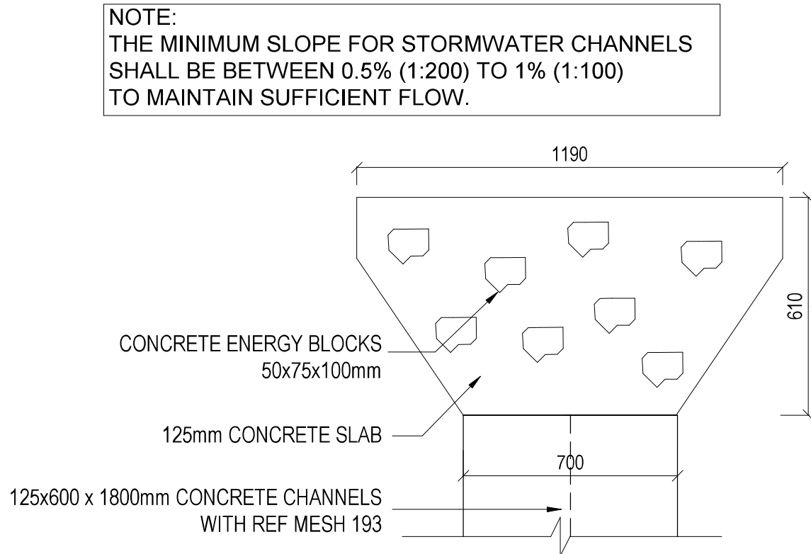
STORM WATER CHANNEL SPREADER SCALE 1:15 (A1)
