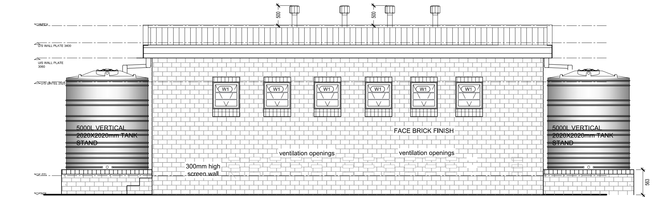
FRONT ELEVATION SCALE 1:50
