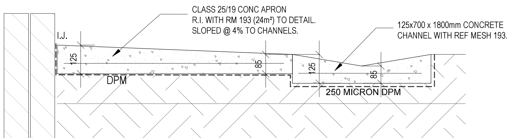
APRON & CHANNEL DETAIL SCALE 1:10 (A1)
