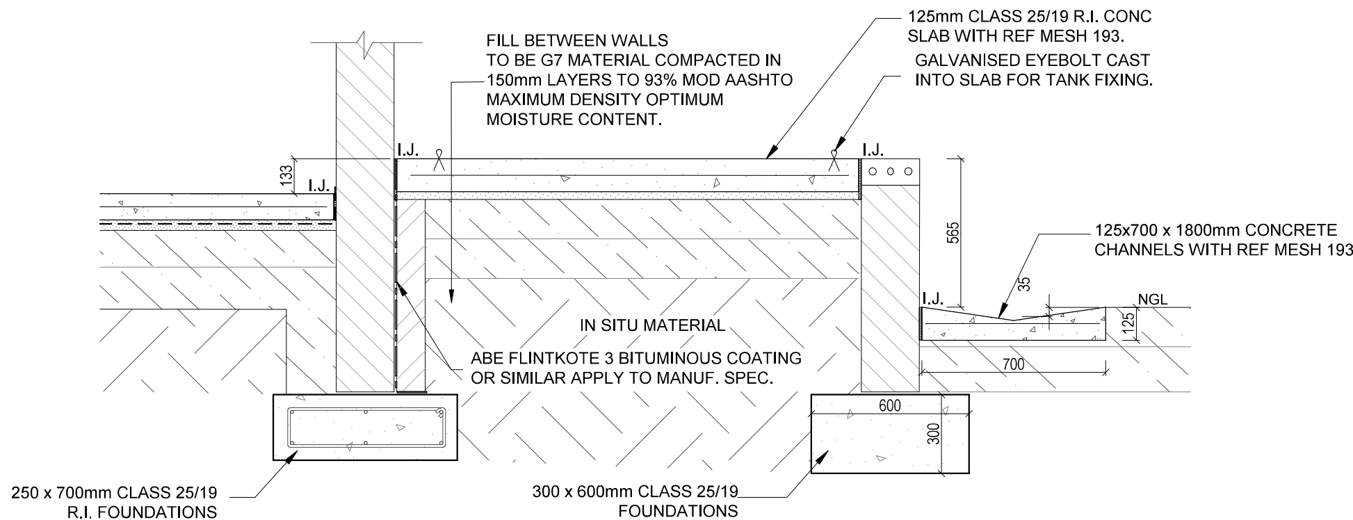
5000lt WATER TANK STAND SECTION SCALE 1:20 (A1)
