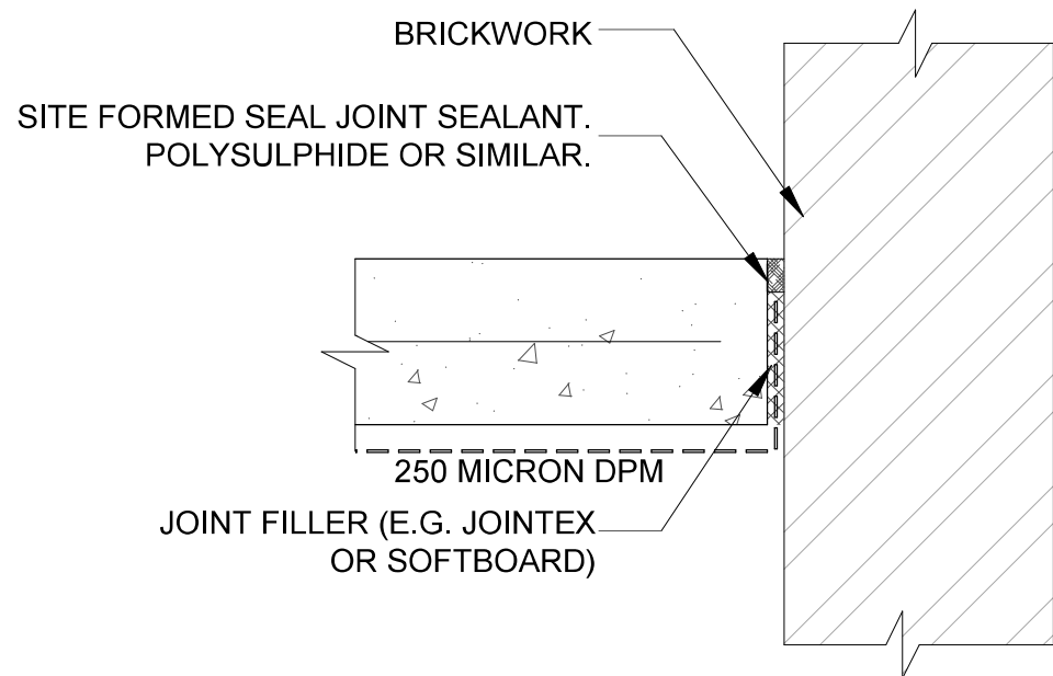
TYPICAL ISOLATION JOINT SCALE 1:5 (A1)
