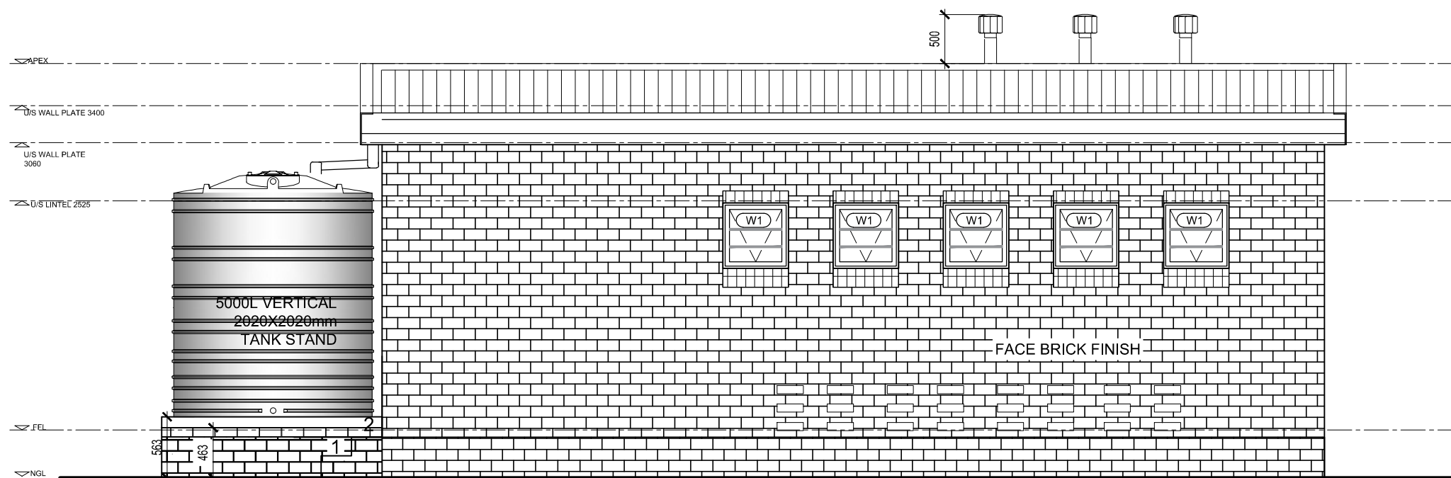
FRONT ELEVATION SCALE 1:50
