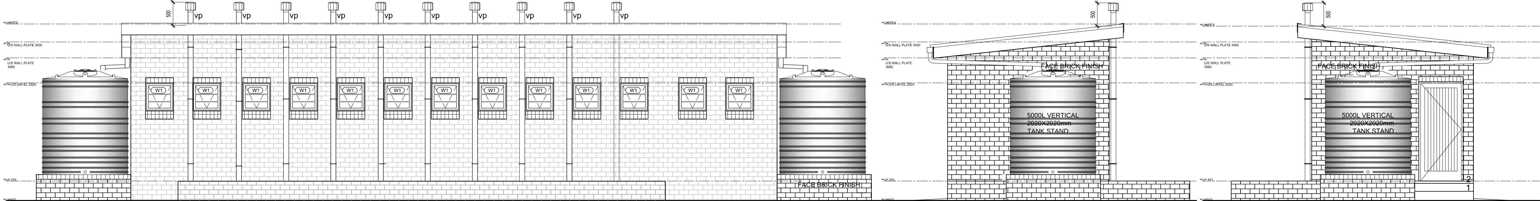
REAR ELEVATION SCALE 1:50
