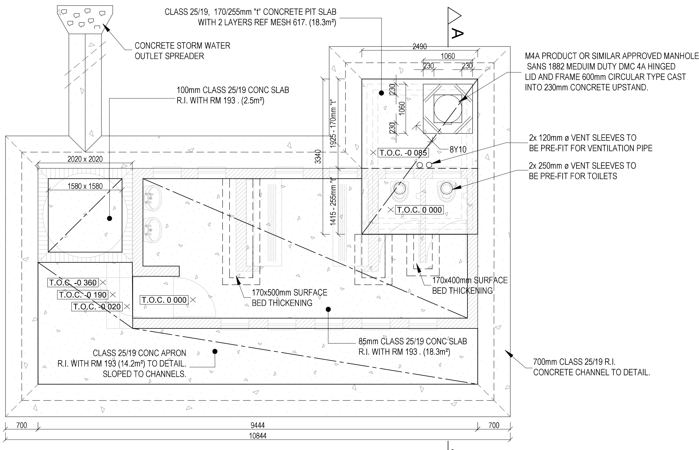
PIT SLAB LAYOUT & SURFACE BED LAYOUT MALE VIP ABLUTIONS
