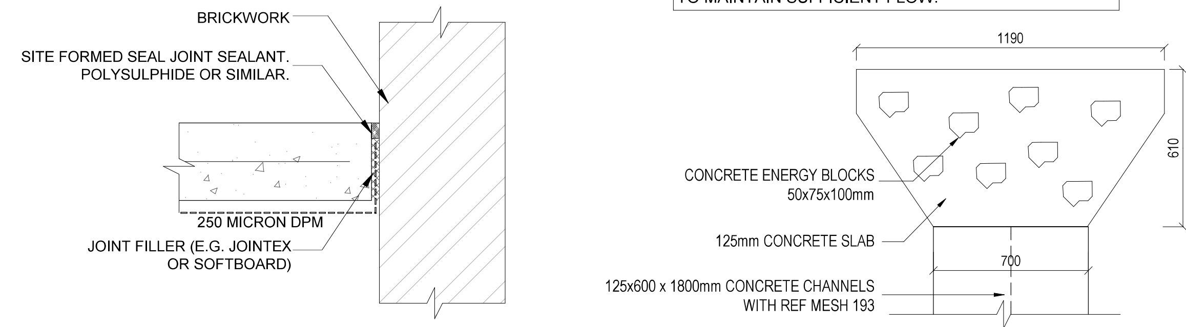
STORM WATER CHANNEL SPREADER SCALE 1:15 (A1)
