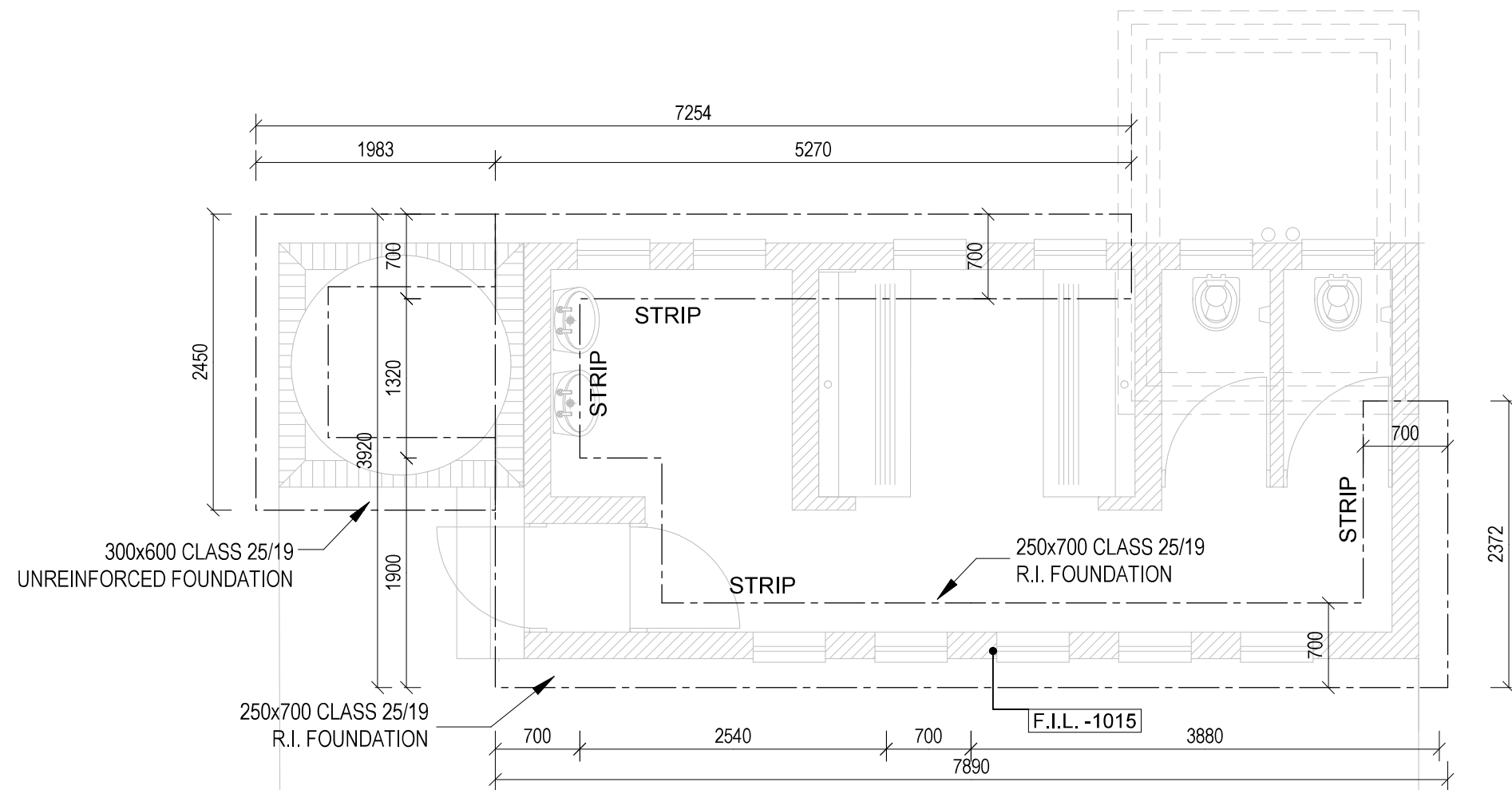
FOUNDATION LAYOUT MALE VIP ABLUTIONS
