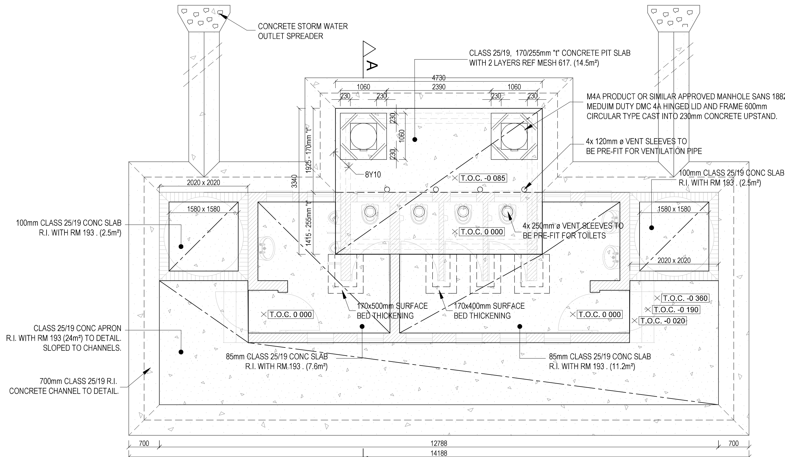
PIT SLAB LAYOUT & SURFACE BED LAYOUT STAFF VIP ABLUTIONS
