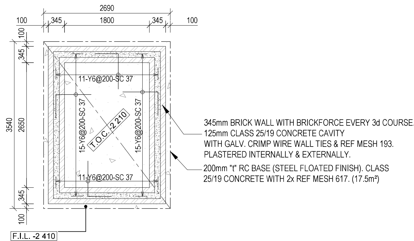
PIT BASE LAYOUT MALE ABLUTIONS
