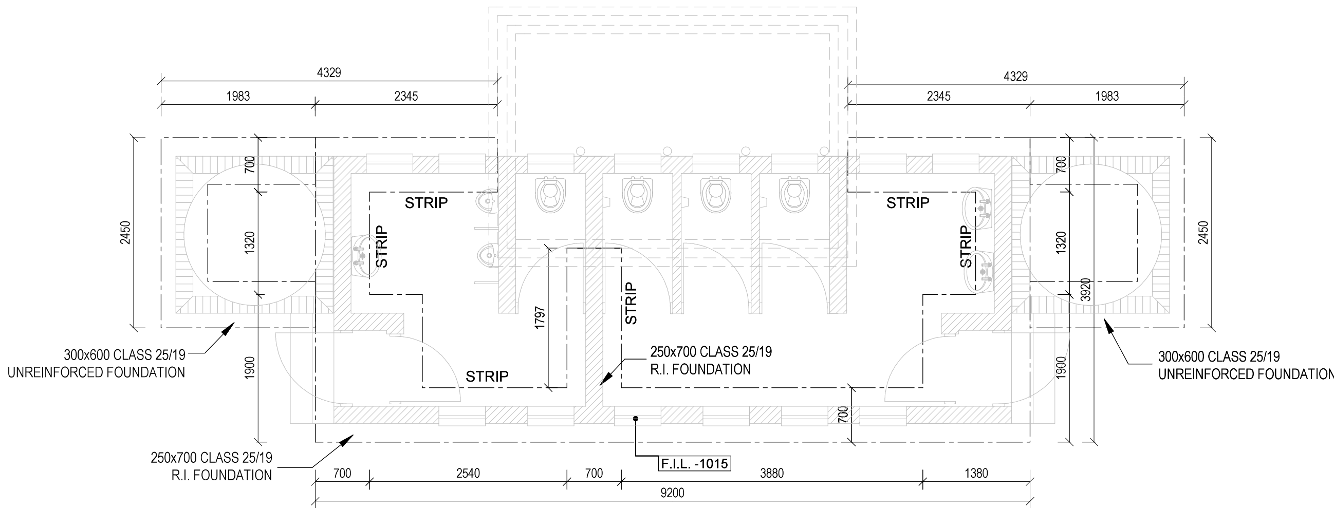
FOUNDATION LAYOUT STAFF VIP ABLUTIONS
